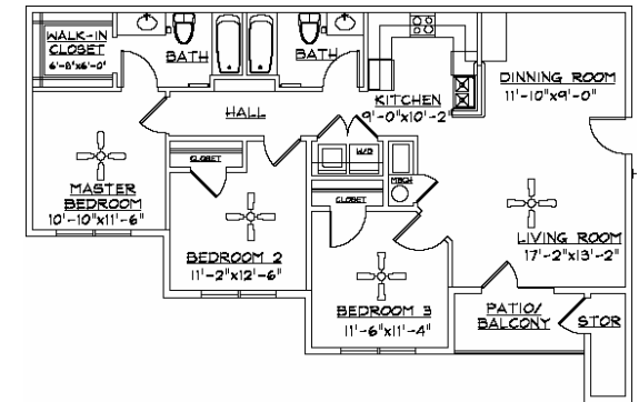
3 Bedroom, 2 Bath Approx. 1300 square feet living space
